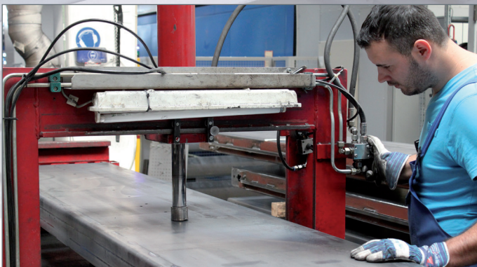
Option "Lowering Device": After welding, the runways for wheel alignment lifts are straightened exactly flat in the area of the turntables and sliding plates.
