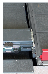
DUO CM in rectangular foundation with (optional) grating, (equipped for vehicle inspection test).
