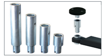
Support disc extensions in five different lengths: 50/100/150/200/300 mm (300 mm only for MA STAR 5.5/6.5)
